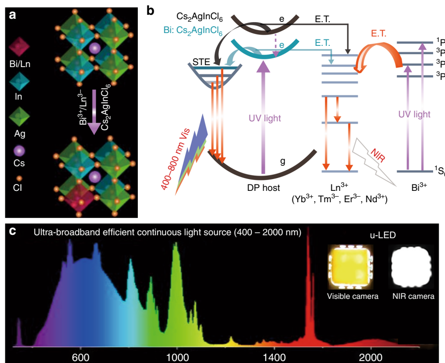
Fig. 1 u-LED relying on the synergy of (STE) recombination and Ln 3+ dopants' 4f–4f transitions of the multi-Ln 3+ -DiG. a Structure diagram of Bi/Ln:Cs 2 AgInCl 6 DPs. b The ultra-broadband emission mechanisms in Bi/Ln:Cs 2 AgInCl 6 DPs. c PL spectrum of the u-LED device. The inset is the photographs of the multi-Ln 3+ -DiG u-LED by visible camera (yellow) and NIR camera (white)
